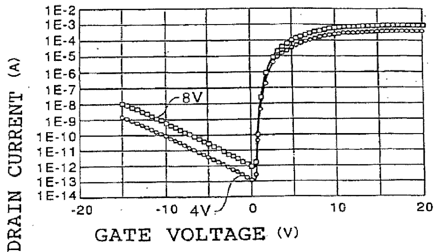
FIG. 11 AMPERE/VOLT CHARACTERISTICS N CHANNEL TYPE TFT
